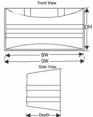
NC-CT36H & NC-CT36 frontal mount side flanges
