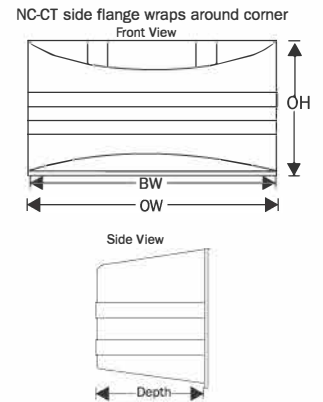
NC-CT36H & NC-CT36 frontal mount side flanges
